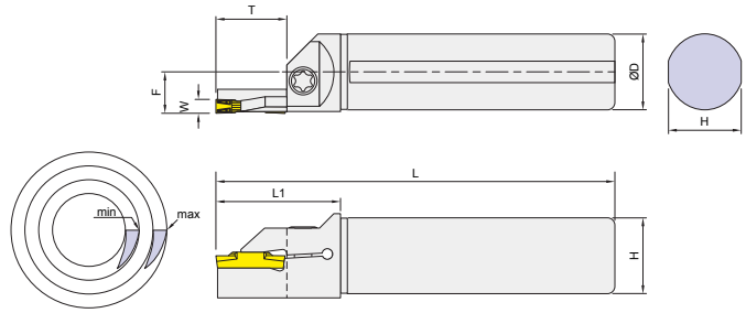
Steel shank (Right-hand shown) 鋼柄 右向示意圖
