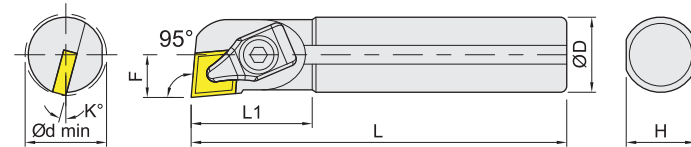
Steel shank (right shown) 鋼柄 右向示意圖
