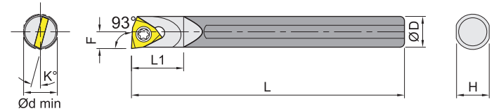
Carbide shank (right shown) 鎢鋼柄 右向示意圖
