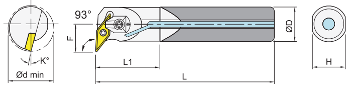
Carbide shank+clamp (right shown) 鎢鋼柄+壓板 右向示意圖
