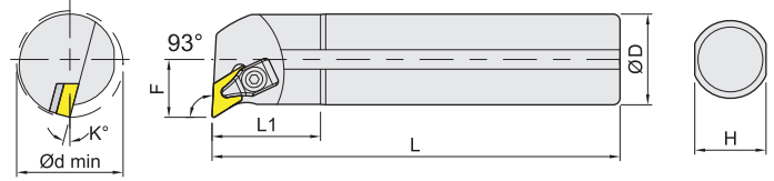
Steel shank (right shown) 鋼柄 右向示意圖
