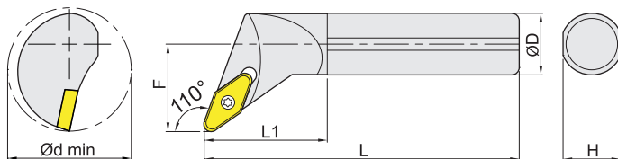
Steel shank (right shown) 鋼柄 右向示意圖
