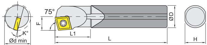
Carbide shank (Right-hand shown) 鎢鋼柄 右向示意圖
